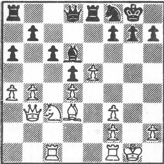
289 After 17 gxf3
